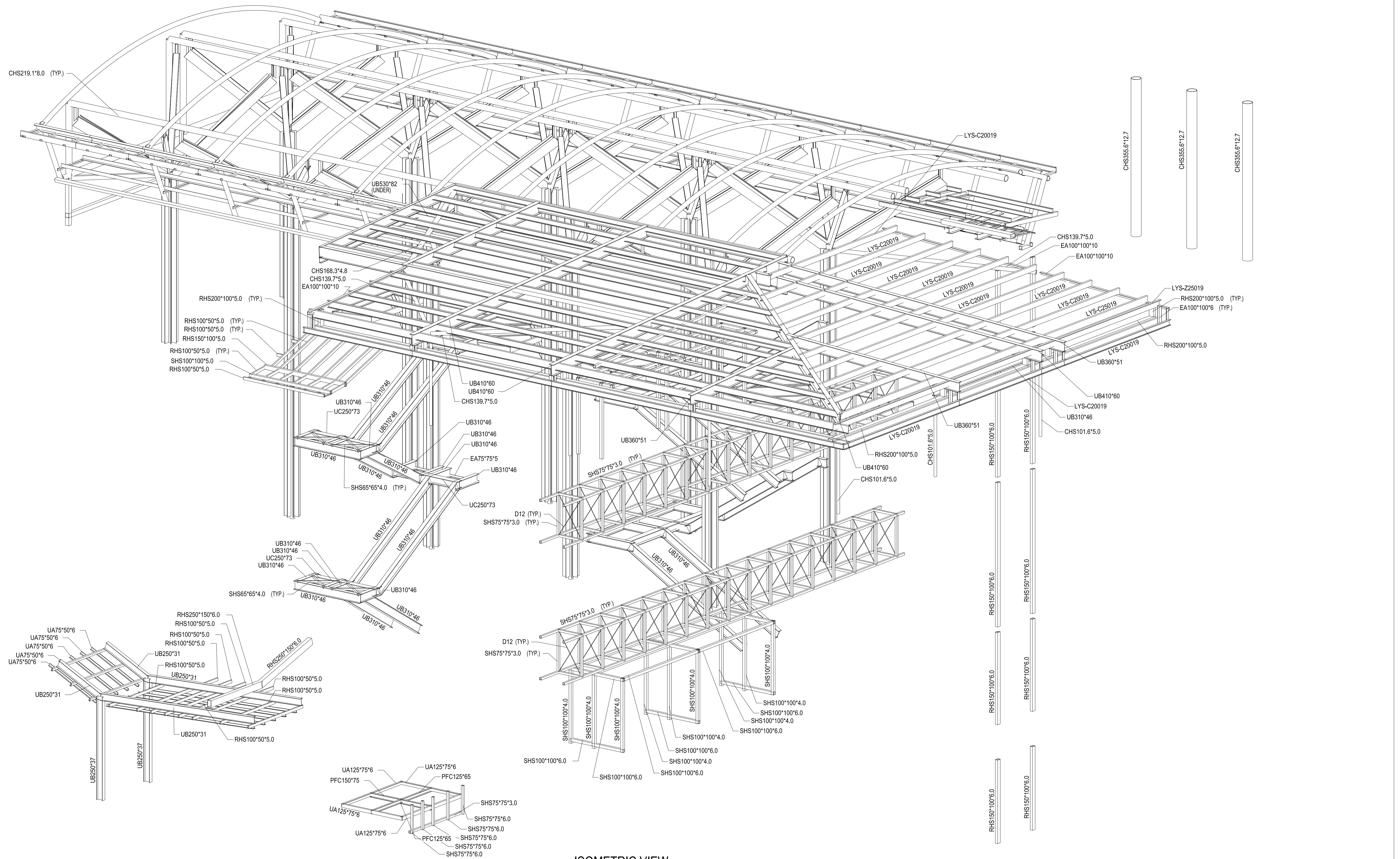
ISOMETRIC VIEW
